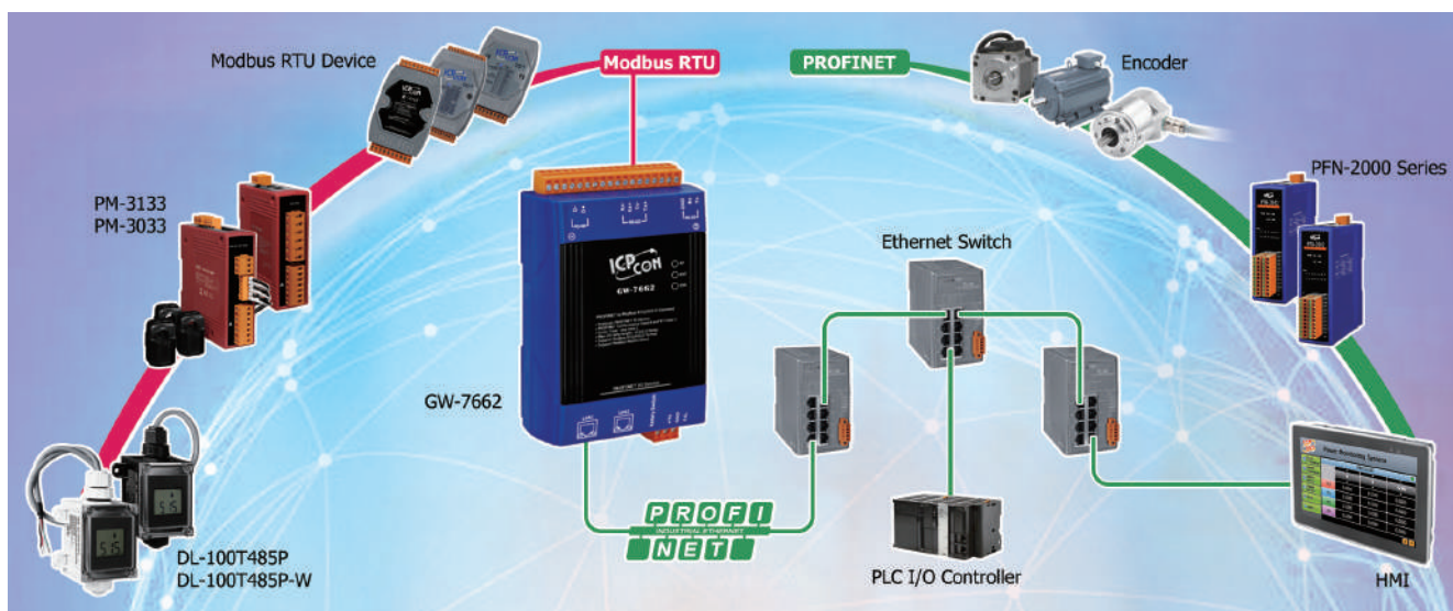
▲GW-7662 can connect PM-3033/3133/3114/3112 device and other ICP DAS's Modbus RTU slave modules in the same time.
