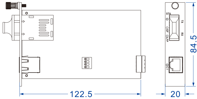
● ECU100M-2GT1GF
