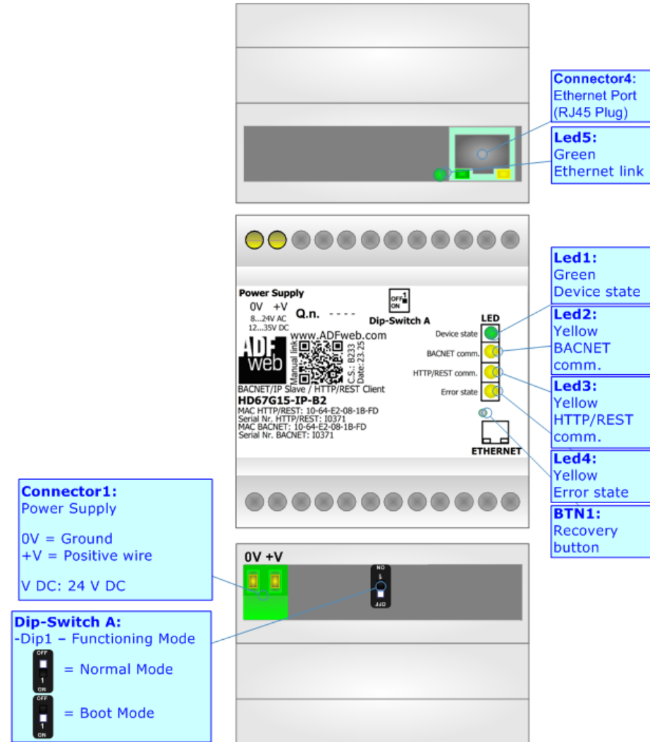
Figure 1a: Connection scheme for HD67G15-IP-B2
