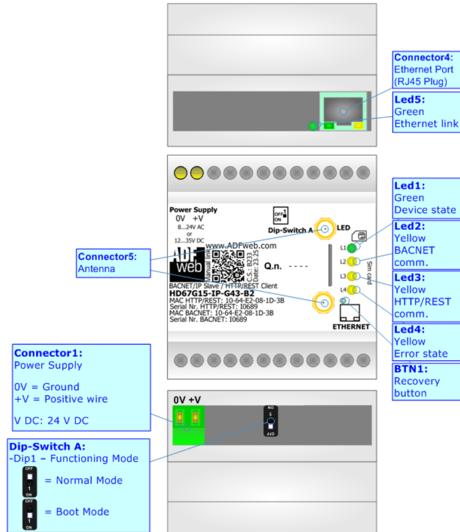
Figure 1b: Connection scheme for HD67G15-IP-G43-x-xxx-B2
