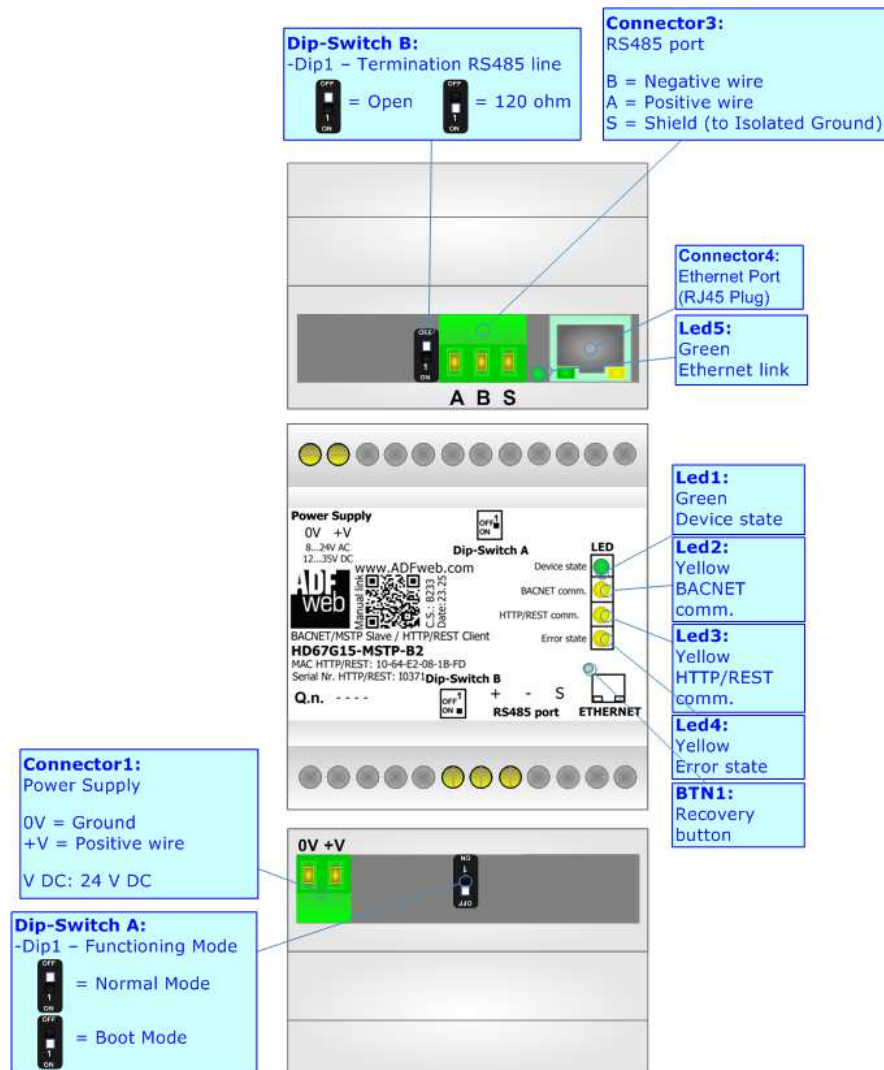
Figure 1c: Connection scheme for HD67G15-MSTP-B2
