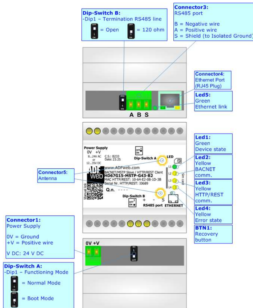
Figure 1d: Connection scheme for HD67G15-MSTP-G43-x-xxx-B2
